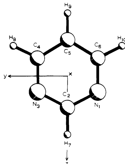
Figure 2. CASSCF-optimized geometry of pyrimidine in its ground state. Also given are the numbering of the atoms and the axis system used.
