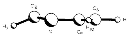
Figure 4. CASSCF-optimized geometry of pyrimidine in the {}^3A_2(n\pi^*) state under the restriction of C_{1h} symmetry. The conformation has been drawn as a projection on the zx plane.
